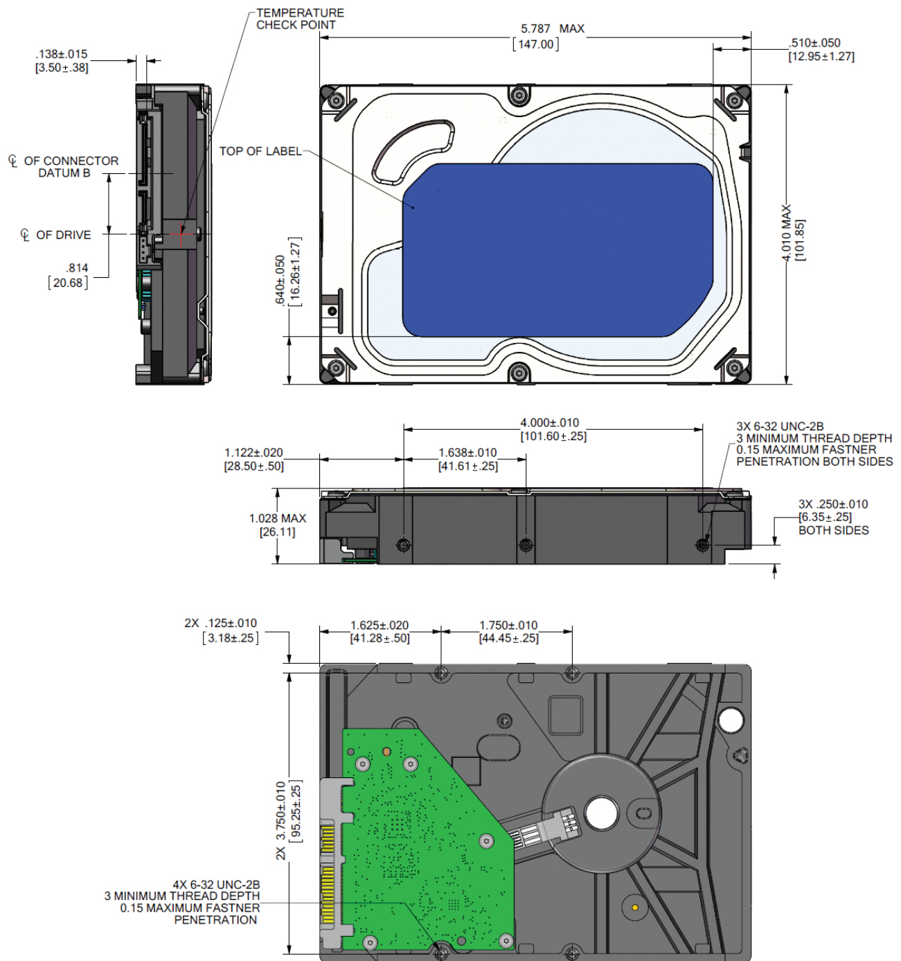
Figure 4 Mounting dimensions (ST4000VN008, ST4000VN006 & ST3000VN006 models)
