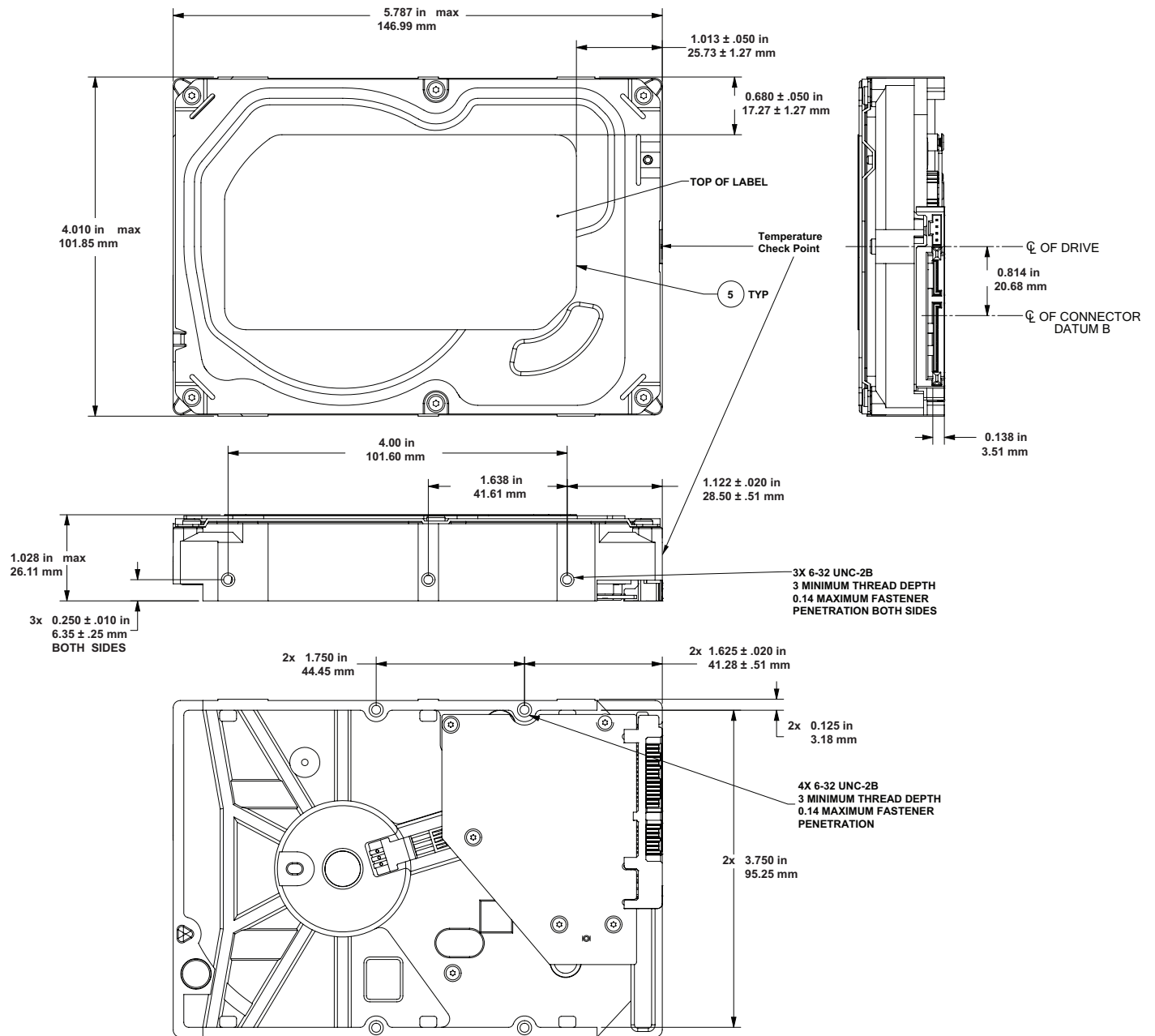
Figure 5 Mounting dimensions (ST3000VN007 & ST2000VN004 models)
