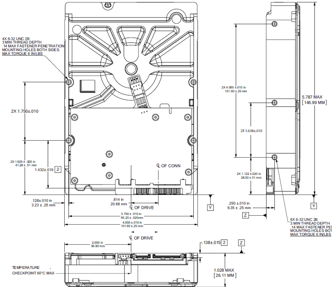
Figure 3 Mounting dimensions (6TB)
