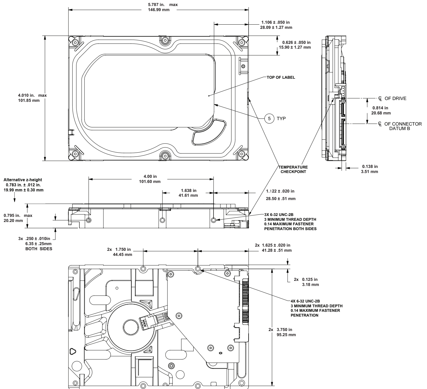
Figure 6 Mounting dimensions (1TB)
